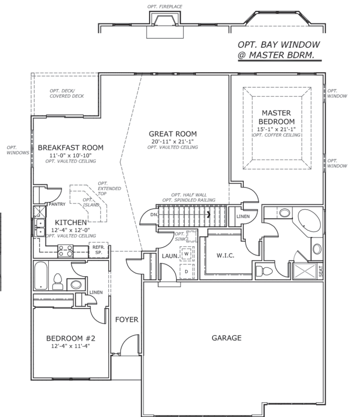
FIRST FLOOR PLAN - 2 BEDROOM w/ OPT. EXTENDED PLAN/ 3 CAR GARAGE
