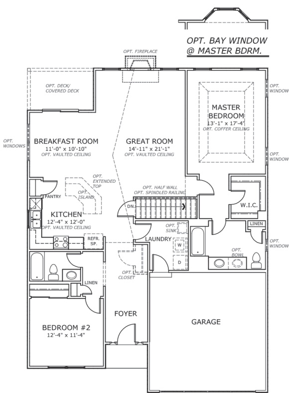
FIRST FLOOR PLAN - 2 BEDROOM
