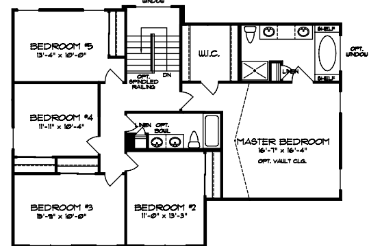
OPT. 2ND FLOOR PLAN (5 B.R.)
