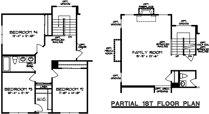
2ND FLOOR PLAN W/ OPT. EXT. FAM. RM.
